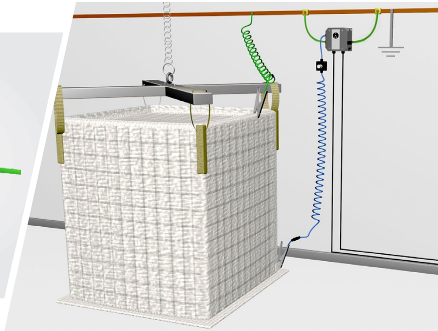
Typical Earth-Rite II FIBC installation consisting of two grounding clamps that establish a continuous ground monitoring loop with the site's locally verified true earth ground source.
